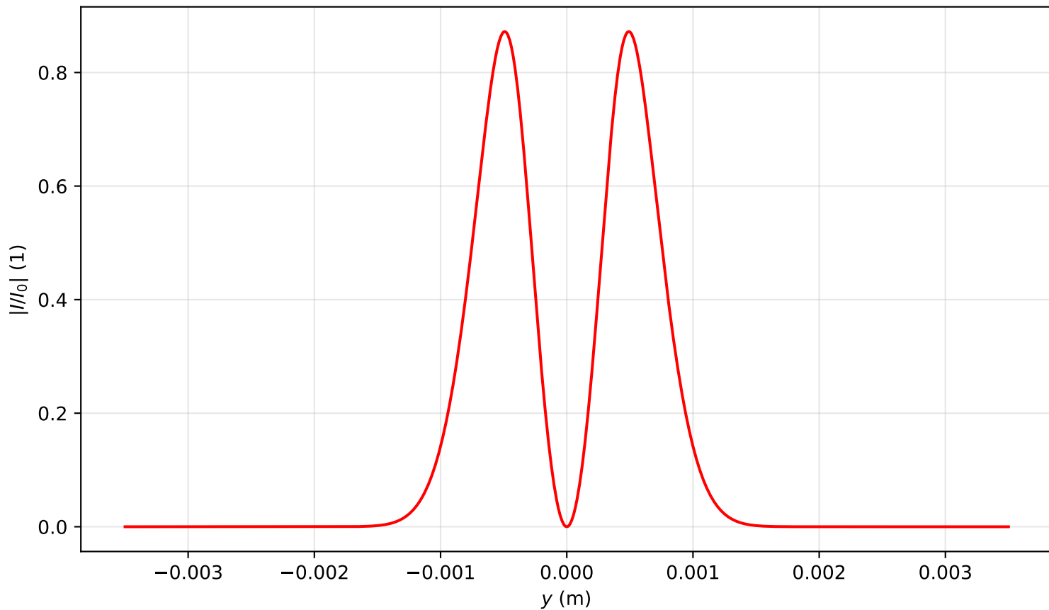
Intensity profile I(x=0, y, z=0.080)/I_0 , P_{in}=16.0P_{cr} , artificial time
