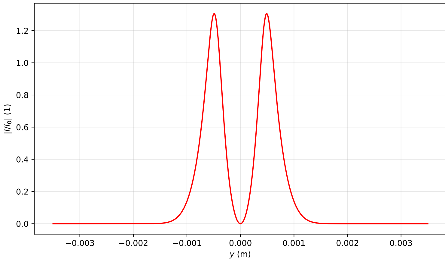
Intensity profile I(x=0, y, z=0.159)/I_0 , P_{in}=16.0P_{cr} , artificial time
