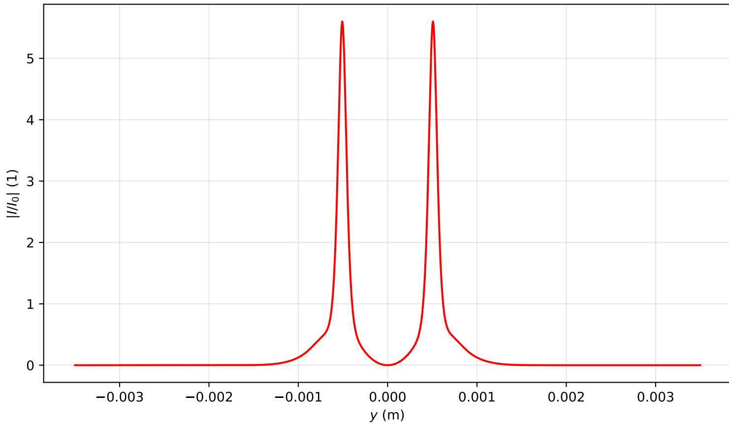
Intensity profile I(x = 0, y, z = 0.318)/I_0 , P_{in}=16.0P_{cr} , artificial time
