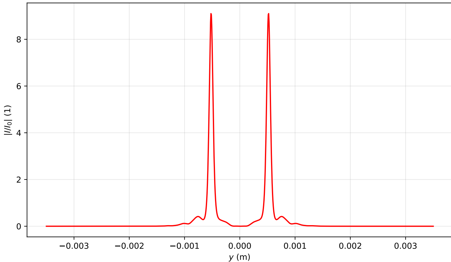
Intensity profile I(x=0, y, z=0.478)/I_0 , \text{Pin}=16.0\text{Pcr} , artificial time
