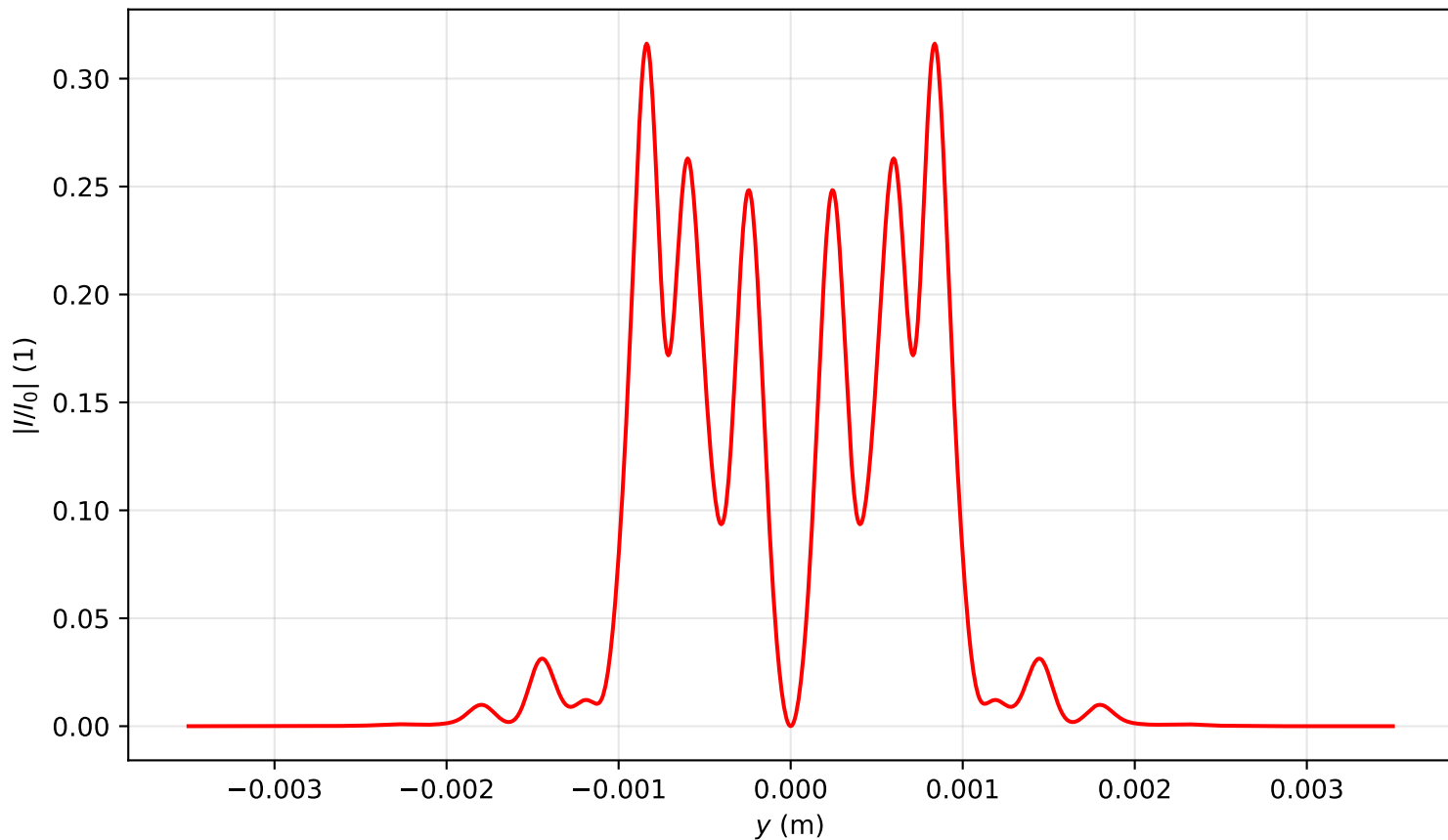
Intensity profile I(x=0, y, z=0.796)/I_0 , P_{in}=16.0\text{Pcr} , artificial time
