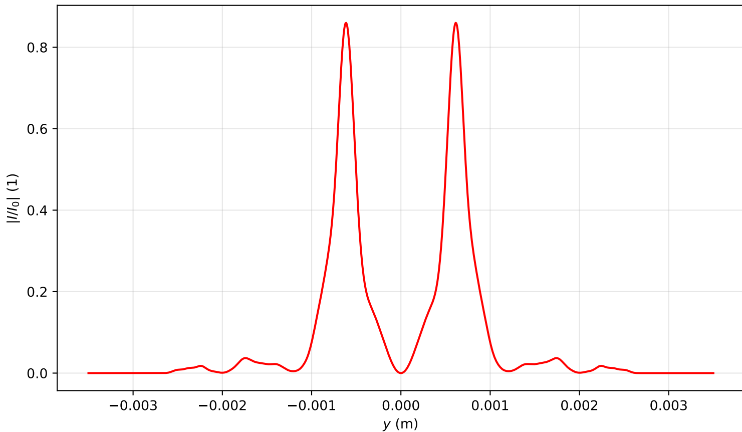
Intensity profile I(x=0, y, z=1.433)/I_0 , P_{in}=16.0P_{cr} , artificial time
