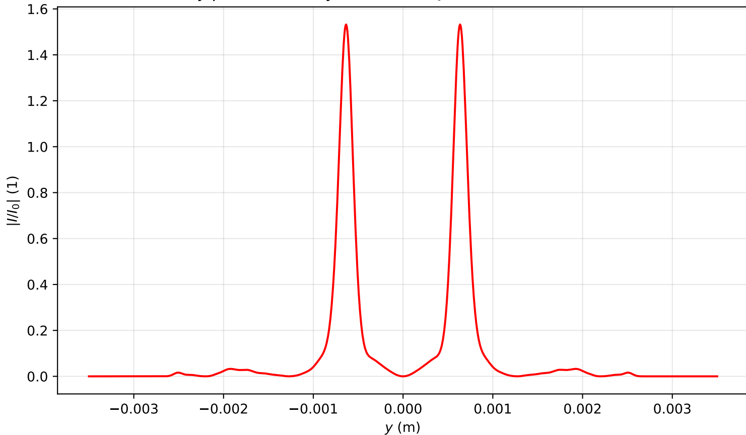
Intensity profile I(x=0, y, z=1.513)/I_0 , P_{in}=16.0P_{cr} , artificial time
