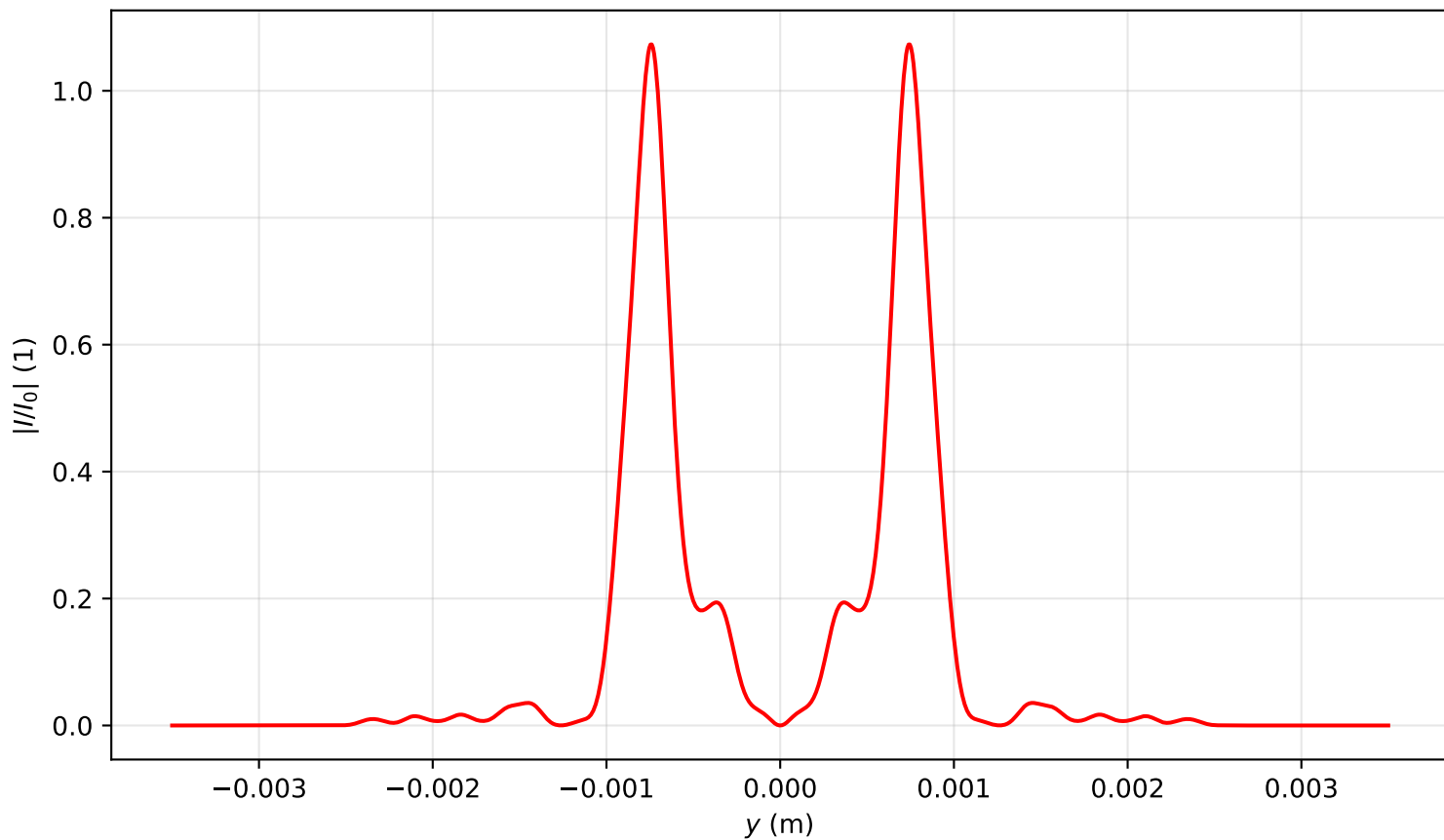
Intensity profile I(x=0, y, z=1.990)/I_0 , P_{in}=16.0P_{cr} , artificial time
