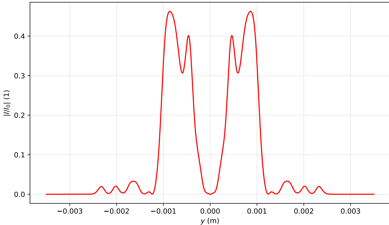
Intensity profile I(x=0, y, z=2.070)/I_0 , P_{in}=16.0P_{cr} , artificial time
