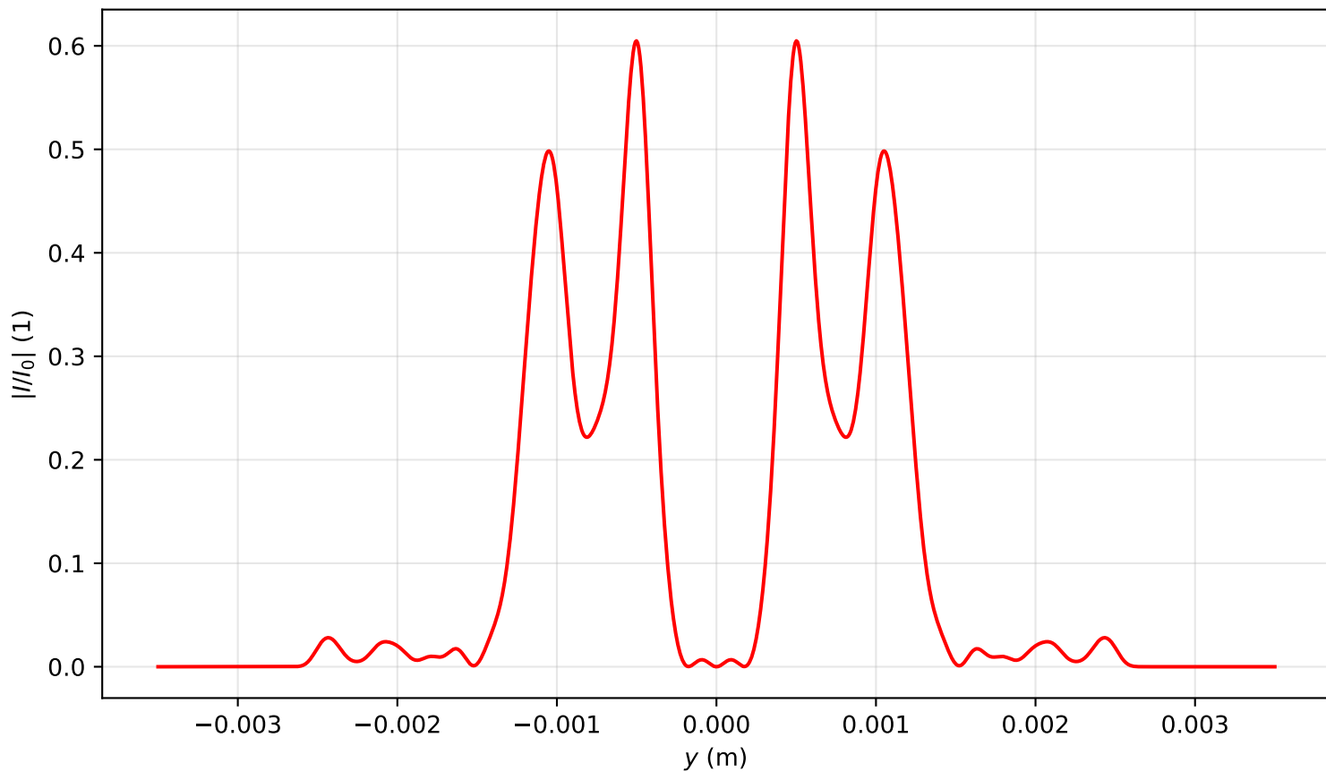
Intensity profile I(x=0, y, z=2.309)/I_0 , P_{in}=16.0P_{cr} , artificial time
