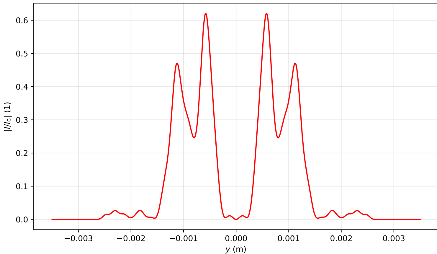
Intensity profile I(x=0, y, z=2.388)/I_0 , P_{in}=16.0P_{cr} , artificial time
