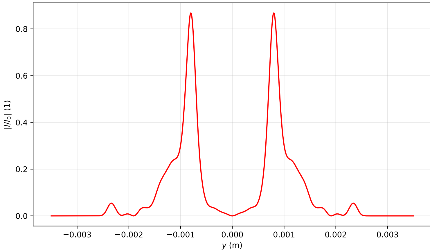
Intensity profile I(x=0, y, z=2.786)/I_0 , P_{in}=16.0P_{cr} , artificial time
