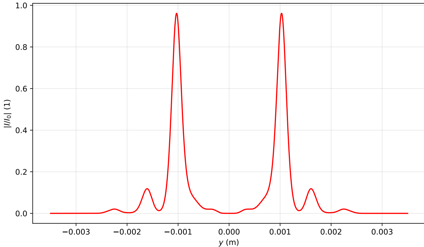
Intensity profile I(x=0, y, z=3.264)/I_0 , P_{in}=16.0P_{cr} , artificial time
