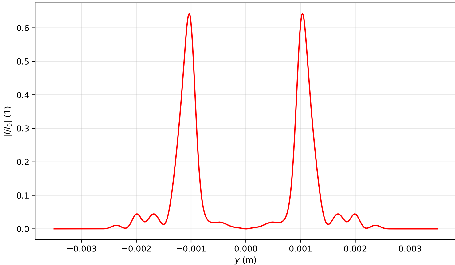
Intensity profile I(x=0, y, z=3.503)/I_0 , P_{in}=16.0P_{cr} , artificial time
