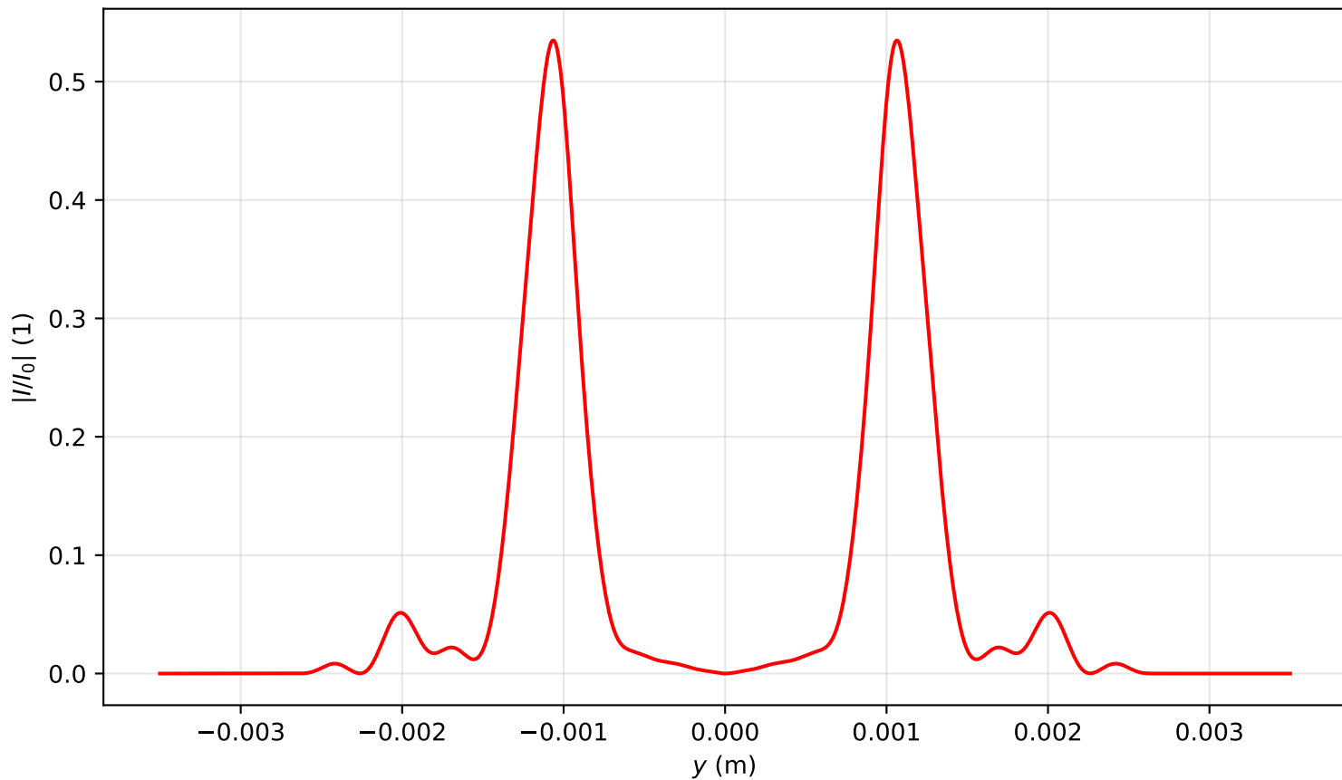
Intensity profile I(x=0, y, z=3.582)/I_0 , P_{in}=16.0P_{cr} , artificial time
