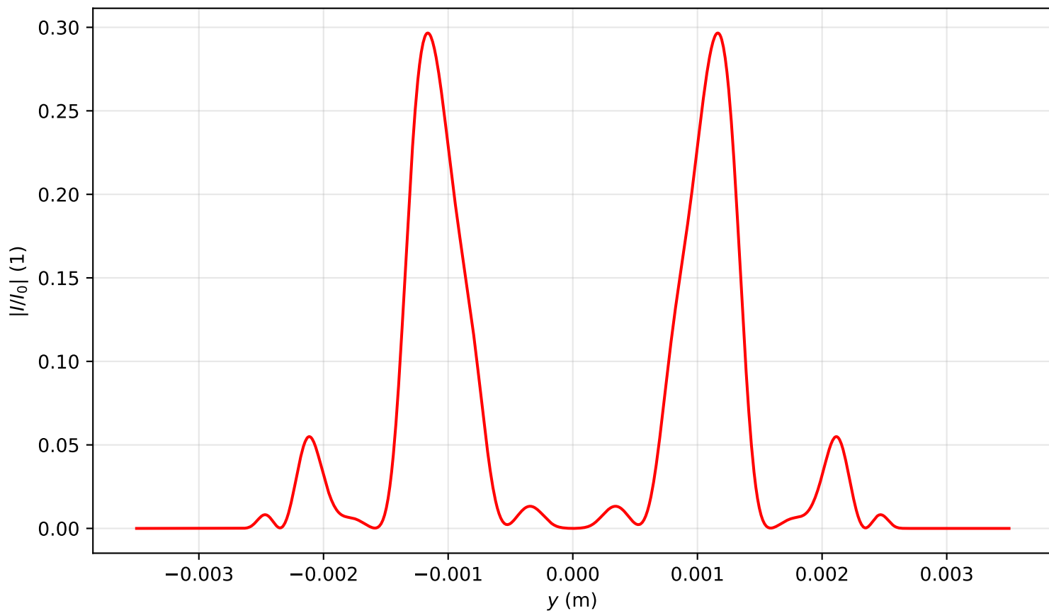
Intensity profile I(x=0, y, z=3.821)/I_0 , P_{in}=16.0\text{Pcr} , artificial time
