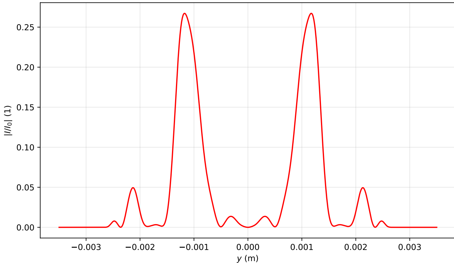
Intensity profile I(x=0, y, z=3.901)/I_0 , P_{in}=16.0\text{Pcr} , artificial time
