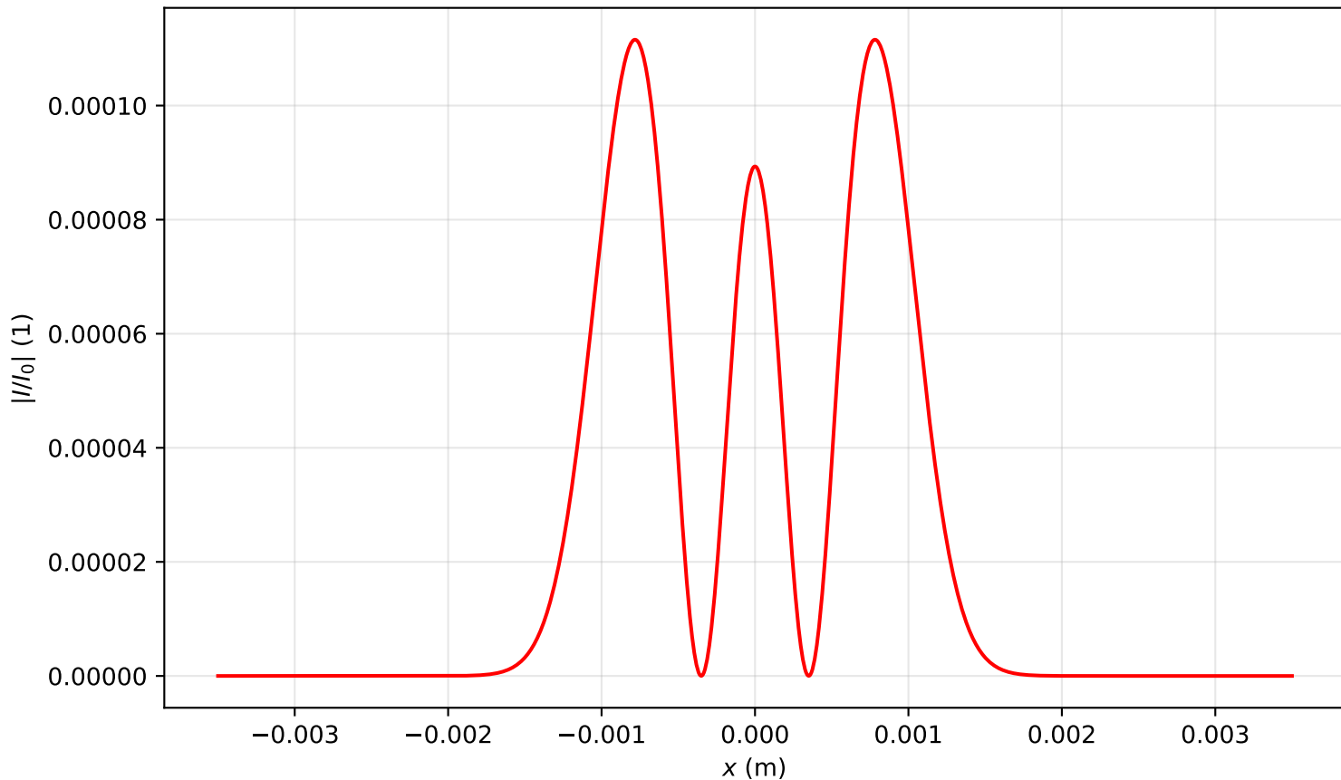
Intensity profile I(x, y = 0, z = 0.080)/I_0 , P_{in}=17.0P_{cr} , artificial time
