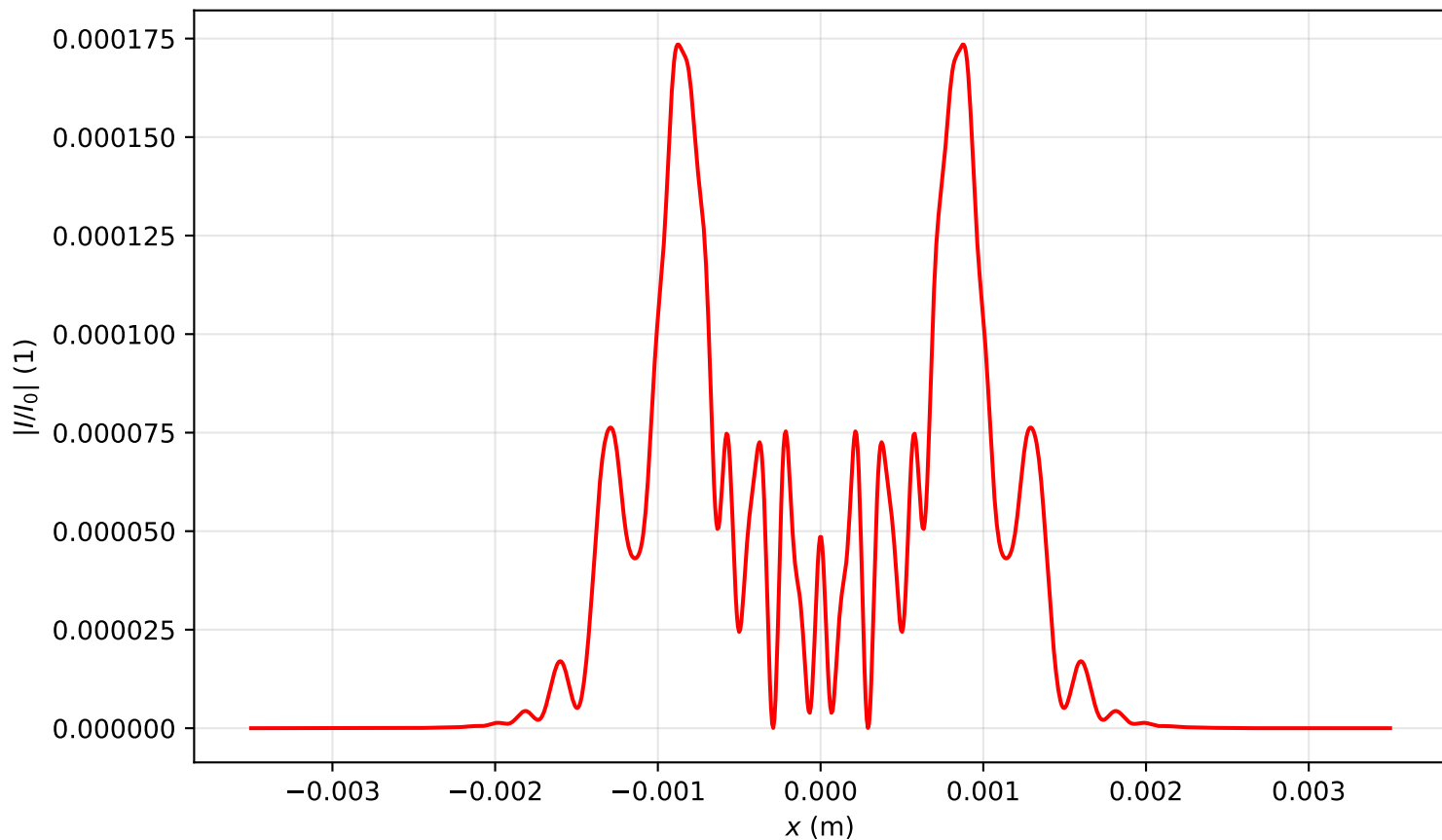
Intensity profile I(x, y = 0, z = 0.478)/I_0 , \text{Pin}=17.0\text{Pcr} , artificial time
