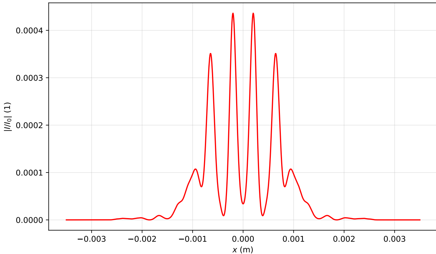
Intensity profile I(x, y = 0, z = 0.876)/I_0 , P_{in}=17.0\text{Pcr} , artificial time
