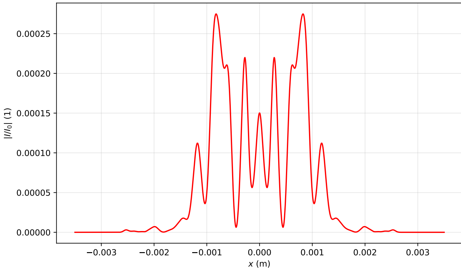
Intensity profile I(x, y = 0, z = 1.035)/I_0 , P_{in}=17.0P_{cr} , artificial time
