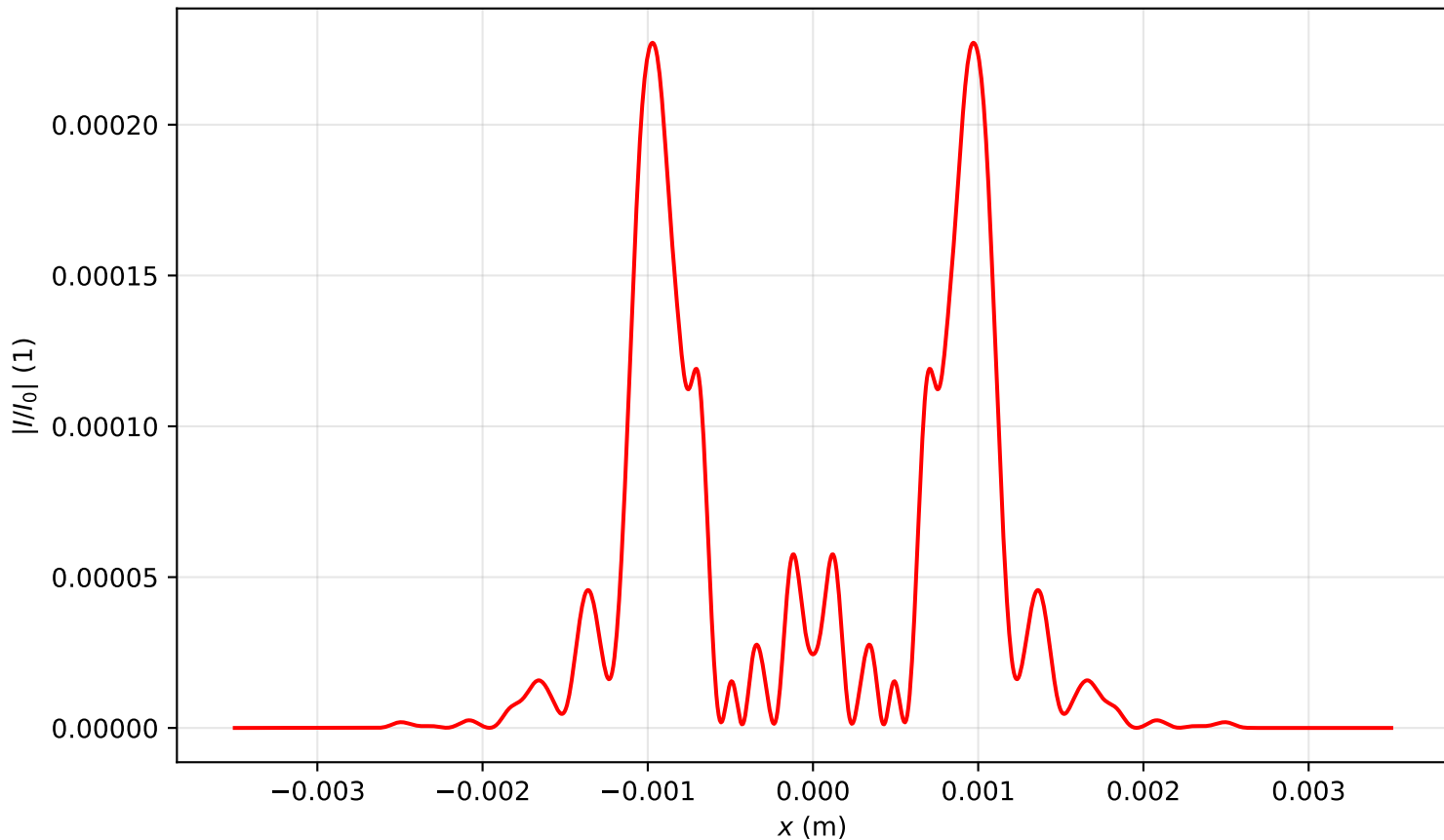
Intensity profile I(x, y = 0, z = 1.353)/I_0 , P_{in}=17.0P_{cr} , artificial time
