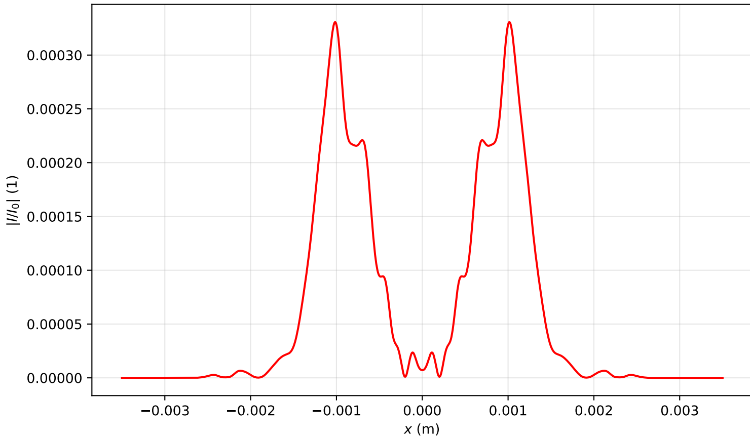
Intensity profile I(x, y = 0, z = 1.513)/I_0 , P_{in}=17.0P_{cr} , artificial time
