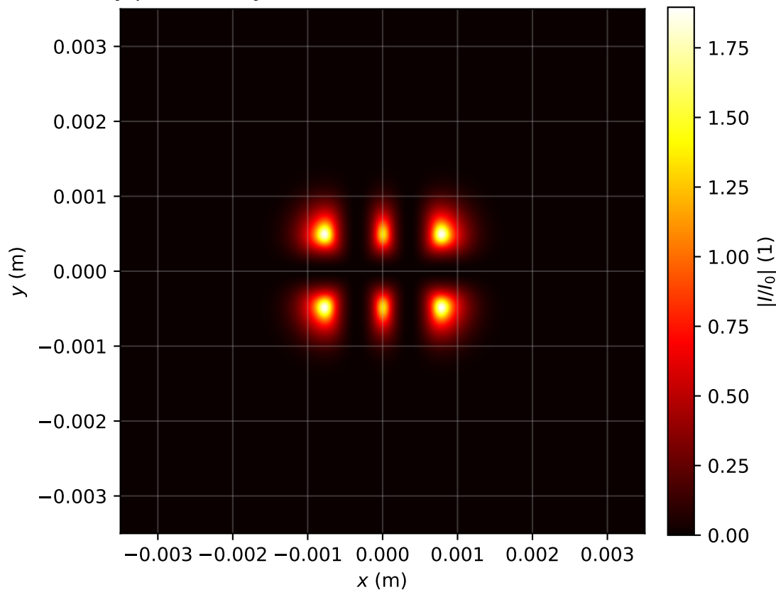
Intensity profile I(x, y, z = 0.159)/I_0 , P_{in}=17.0P_{cr} , artificial time
