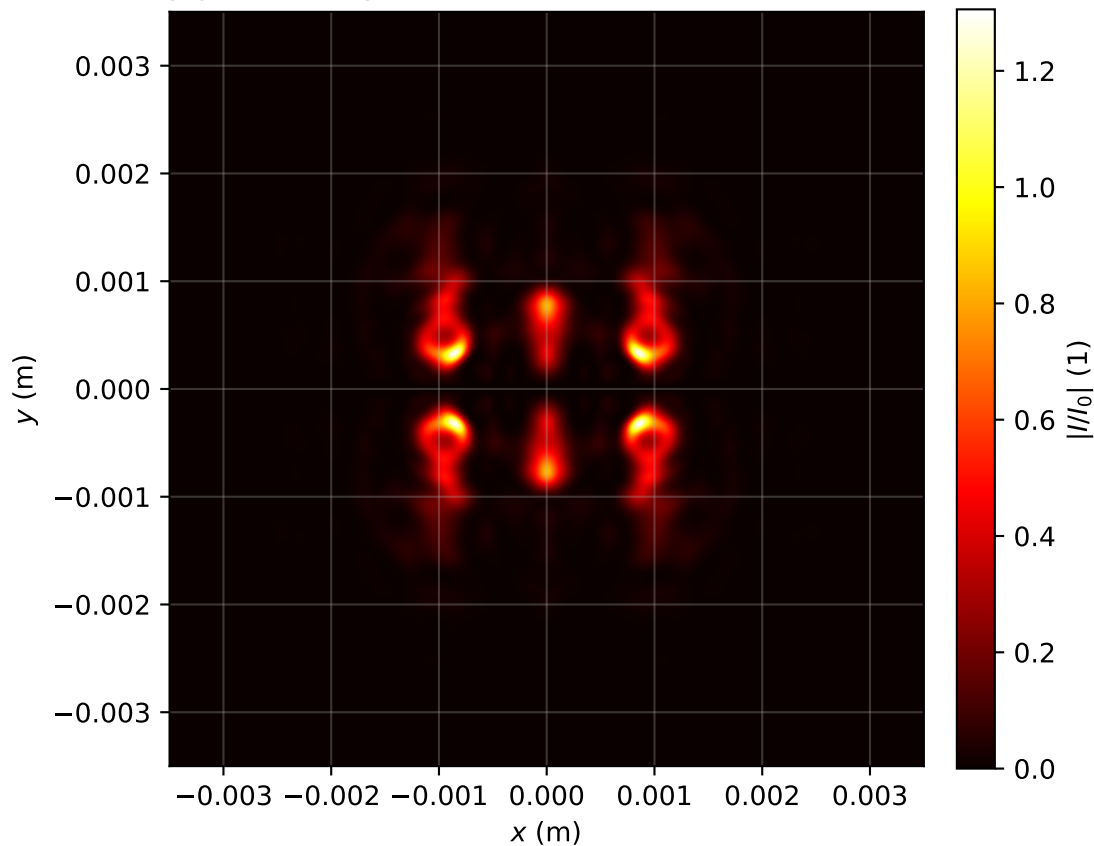
Intensity profile I(x, y, z = 1.274)/I_0 , P_{in}=17.0\text{Pcr} , artificial time
