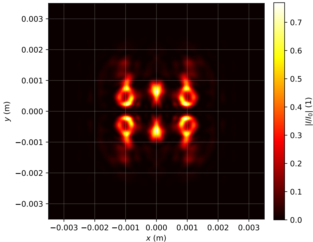
Intensity profile I(x, y, z = 1.353)/I_0 , P_{in}=17.0\text{Pcr} , artificial time
