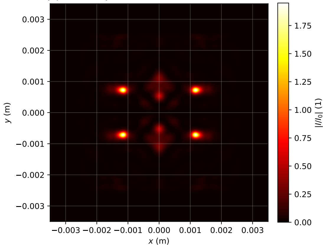
Intensity profile I(x, y, z = 2.229)/I_0 , P_{in}=17.0P_{cr} , artificial time
