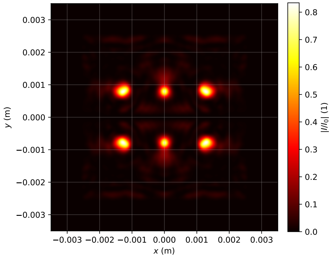
Intensity profile I(x, y, z = 2.627)/I_0 , P_{in}=17.0\text{Pcr} , artificial time
