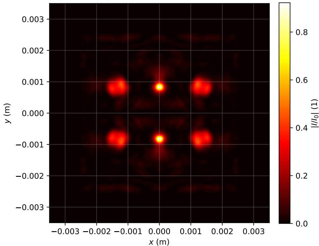
Intensity profile I(x, y, z = 2.707)/I_0 , P_{in}=17.0\text{Pcr} , artificial time
