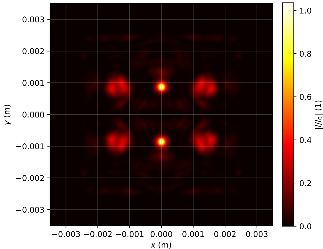
Intensity profile I(x, y, z = 2.786)/I_0 , P_{in}=17.0\text{Pcr} , artificial time
