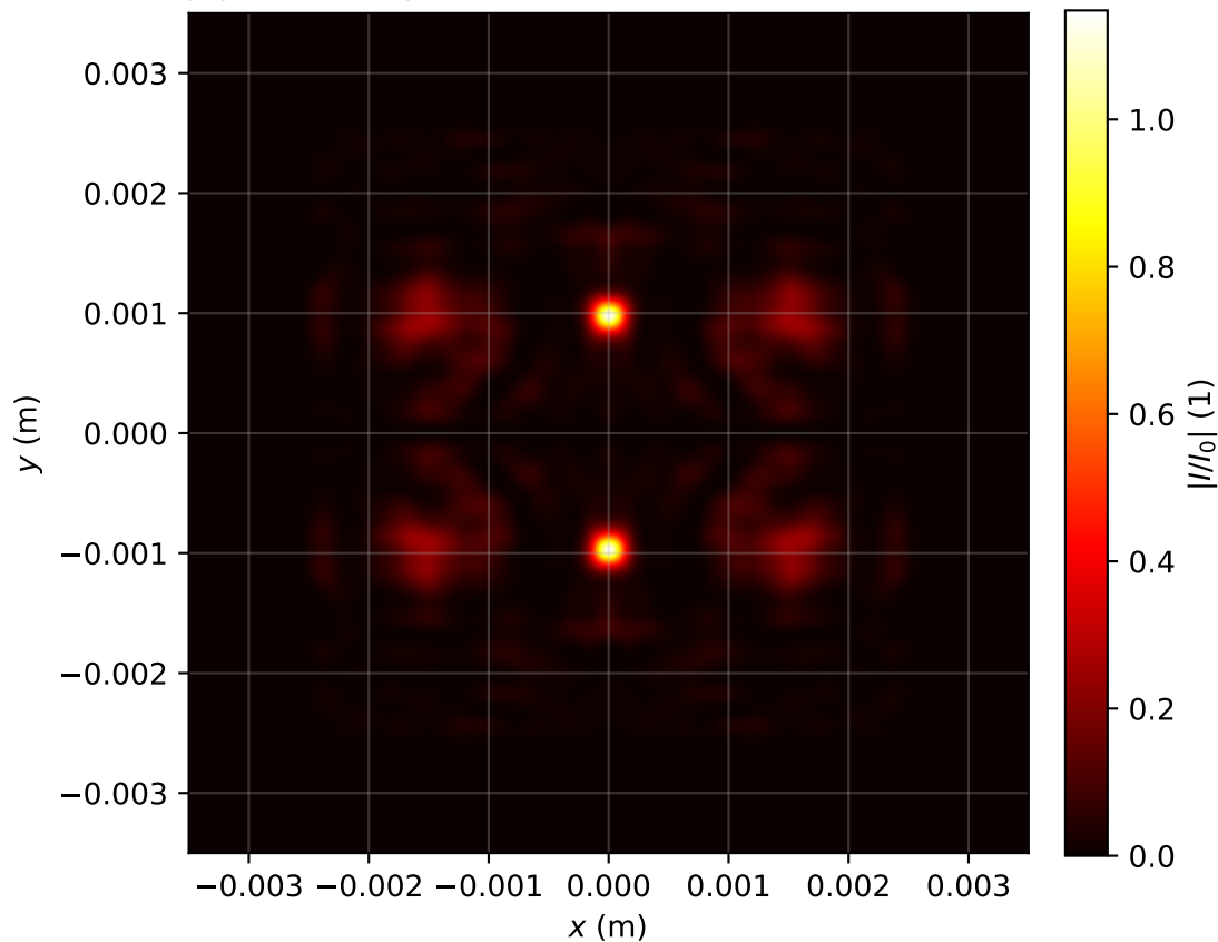
Intensity profile I(x, y, z = 3.025)/I_0 , P_{in}=17.0\text{Pcr} , artificial time
