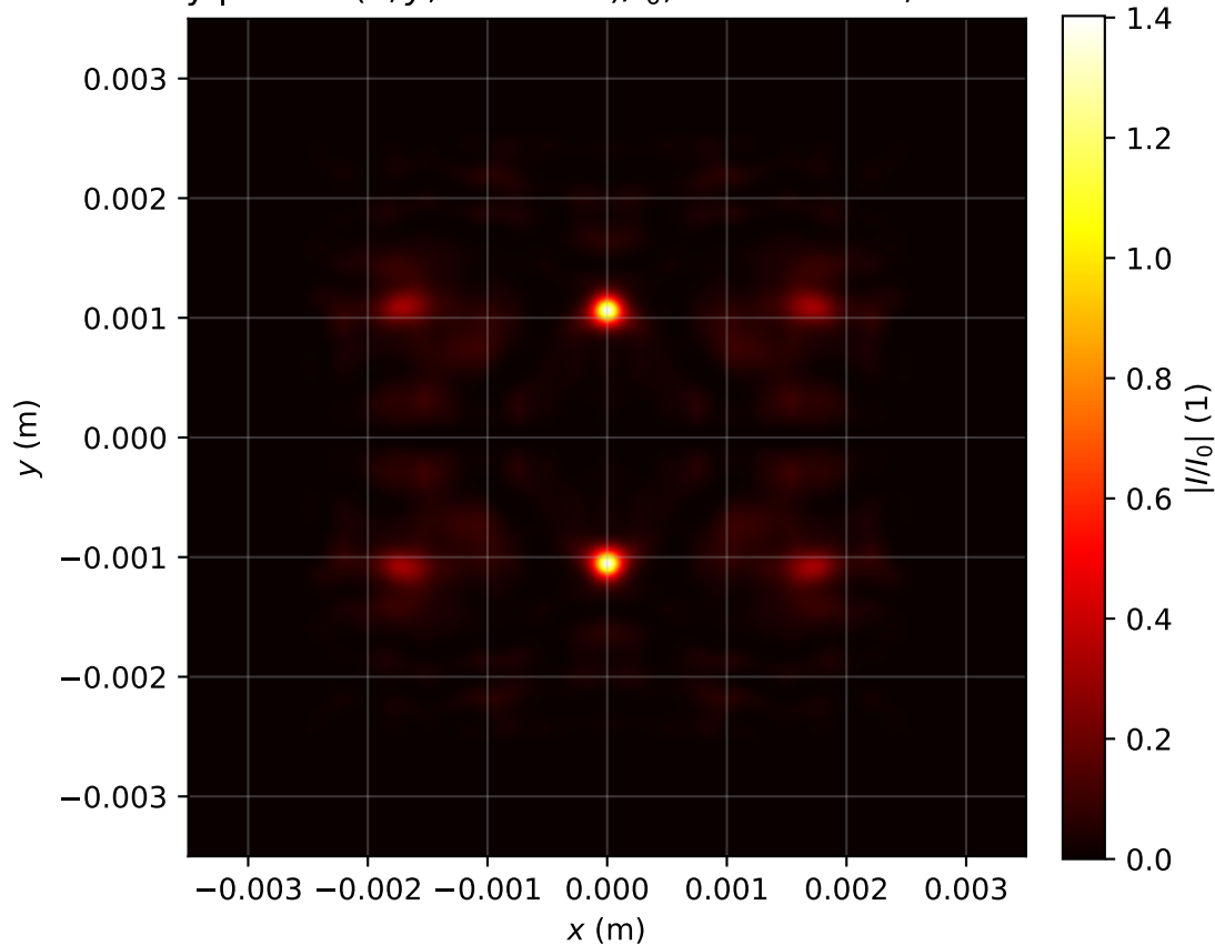
Intensity profile I(x, y, z = 3.344)/I_0 , P_{in}=17.0\text{Pcr} , artificial time
