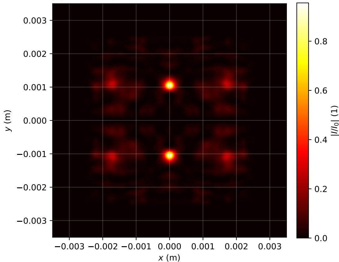
Intensity profile I(x, y, z = 3.423)/I_0 , P_{in}=17.0P_{cr} , artificial time
