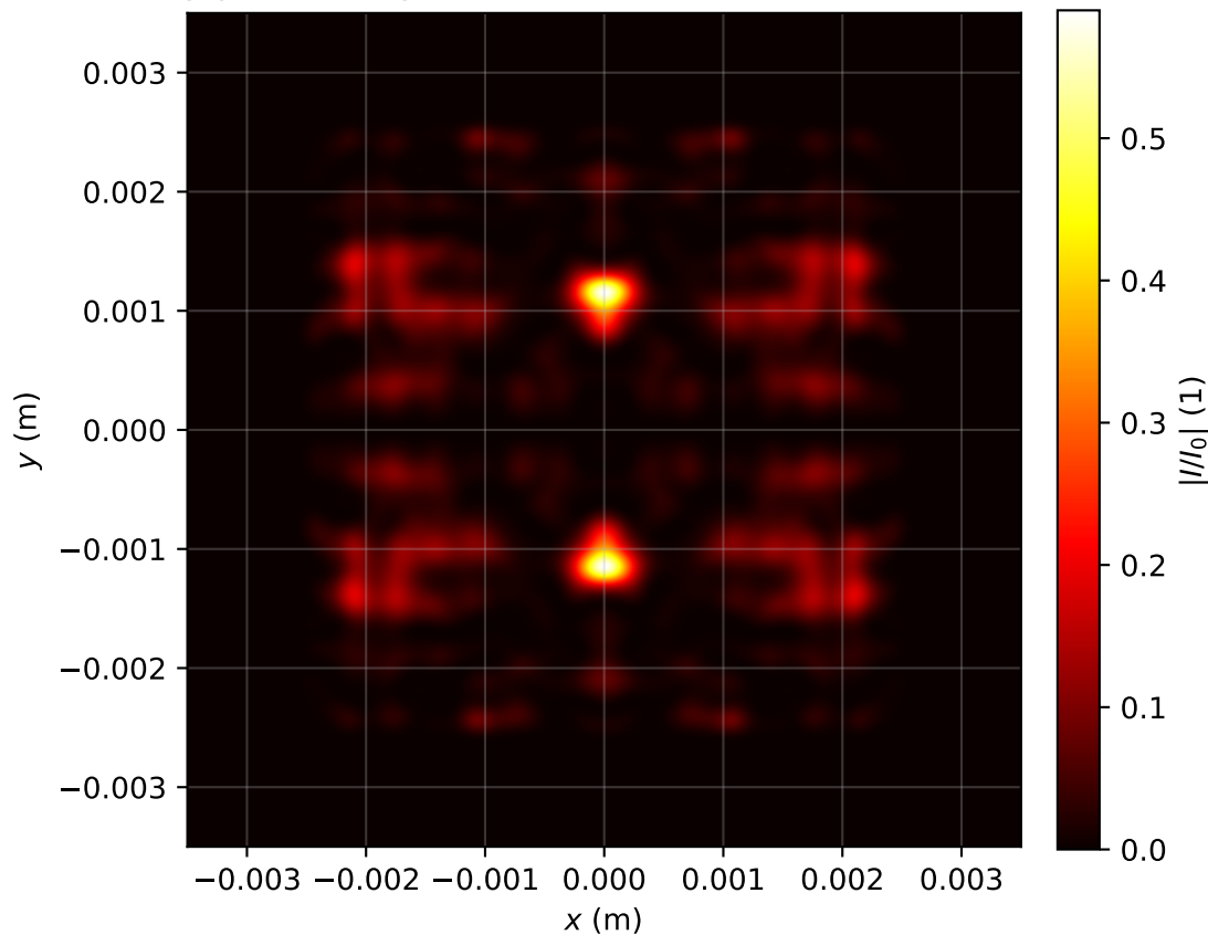
Intensity profile I(x, y, z = 3.662)/I_0 , P_{in}=17.0\text{Pcr} , artificial time
