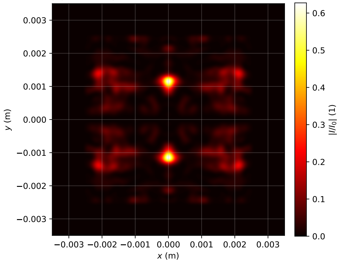
Intensity profile I(x, y, z = 3.742)/I_0 , P_{in}=17.0P_{cr} , artificial time
