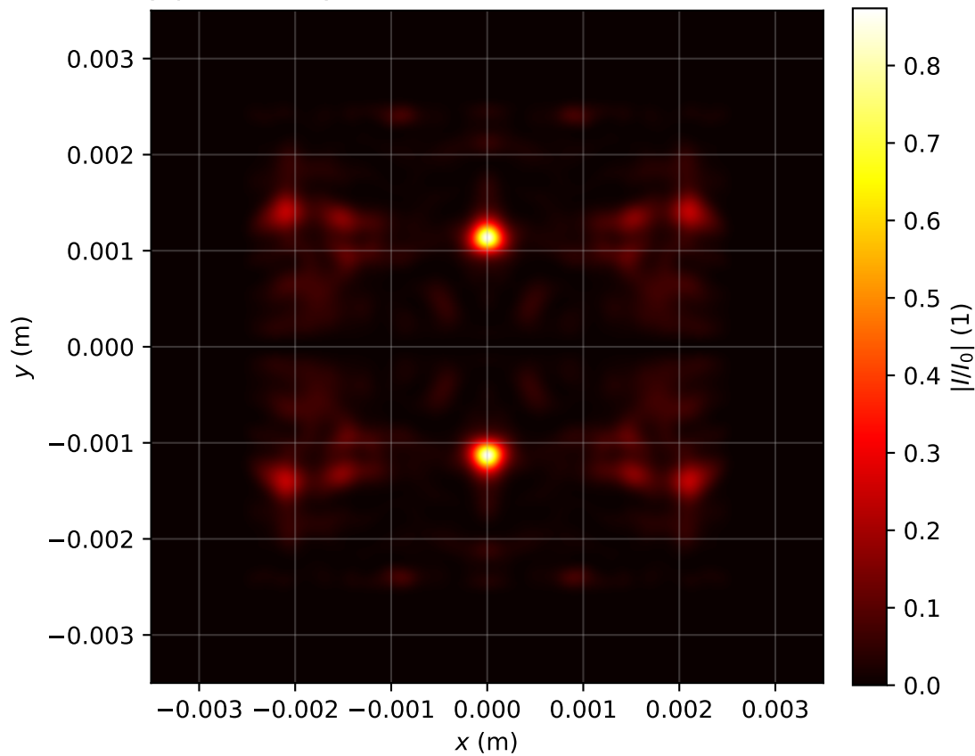
Intensity profile I(x, y, z = 3.901)/I_0 , P_{in}=17.0\text{Pcr} , artificial time
