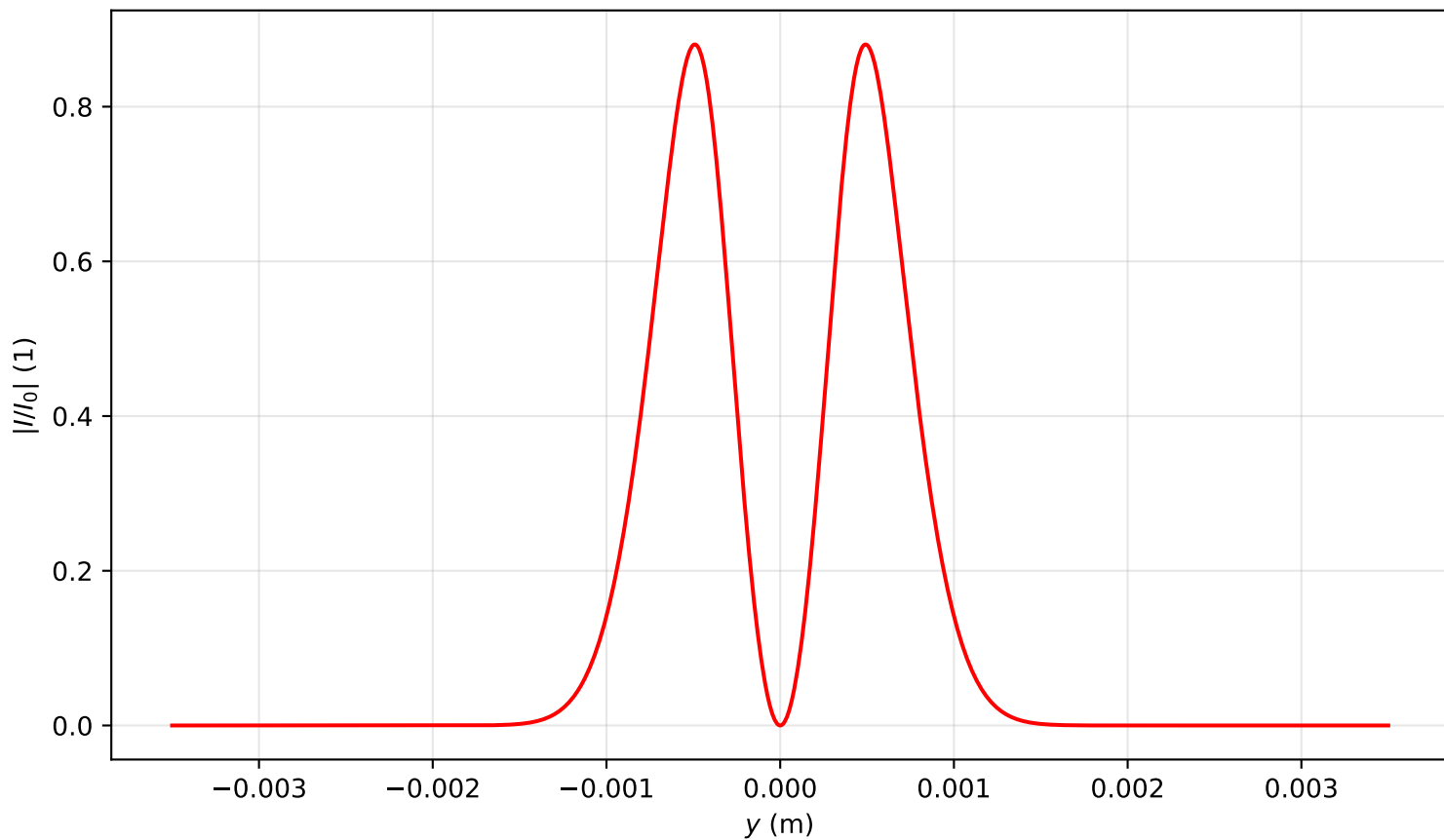
Intensity profile I(x=0, y, z=0.080)/I_0 , P_{in}=17.0P_{cr} , artificial time
