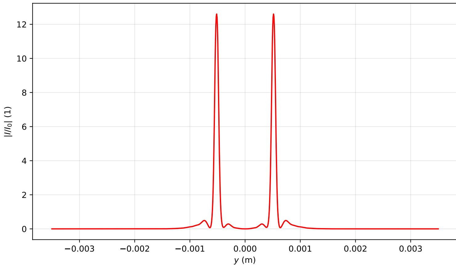
Intensity profile I(x=0, y, z=0.398)/I_0 , P_{in}=17.0P_{cr} , artificial time
