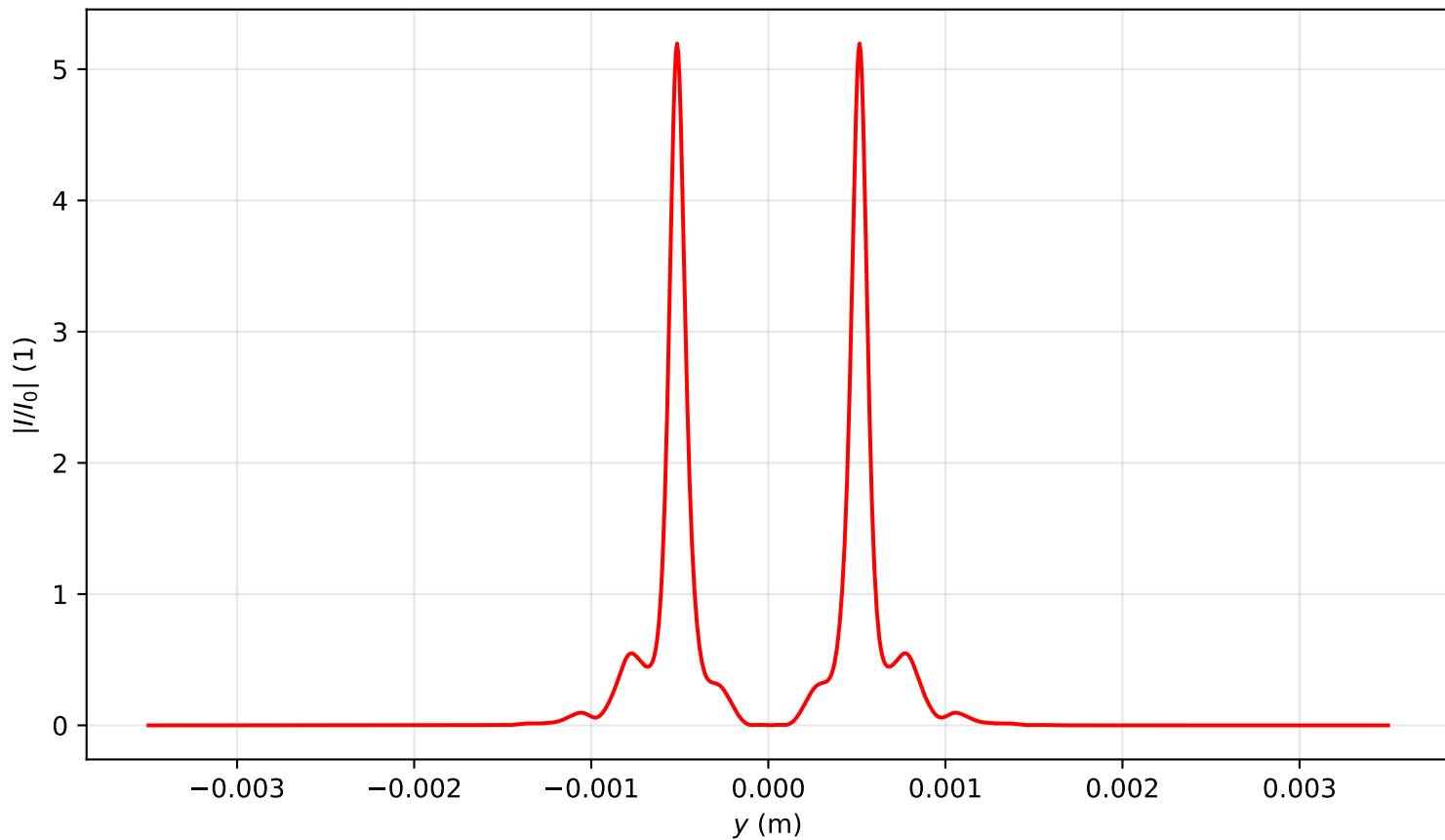
Intensity profile I(x=0, y, z=0.478)/I_0 , P_{in}=17.0P_{cr} , artificial time
