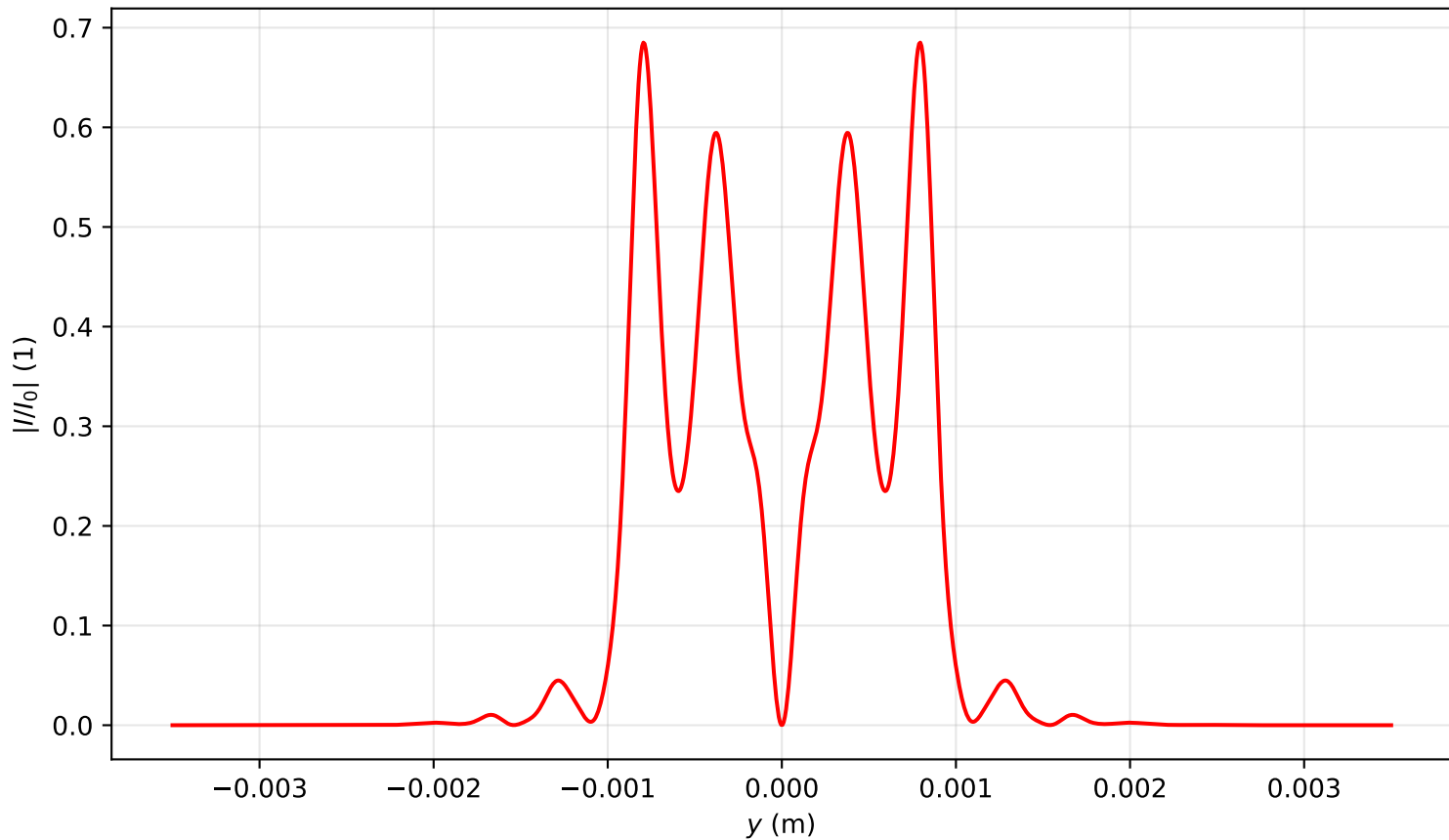
Intensity profile I(x=0, y, z=0.716)/I_0 , P_{in}=17.0\text{Pcr} , artificial time
