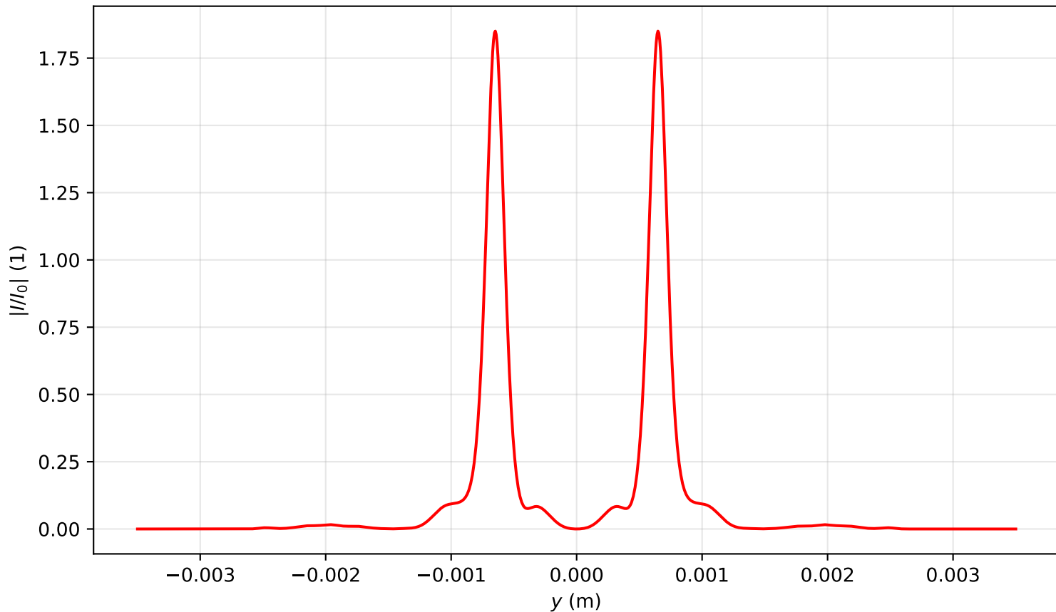
Intensity profile I(x=0, y, z=1.513)/I_0 , P_{in}=17.0P_{cr} , artificial time
