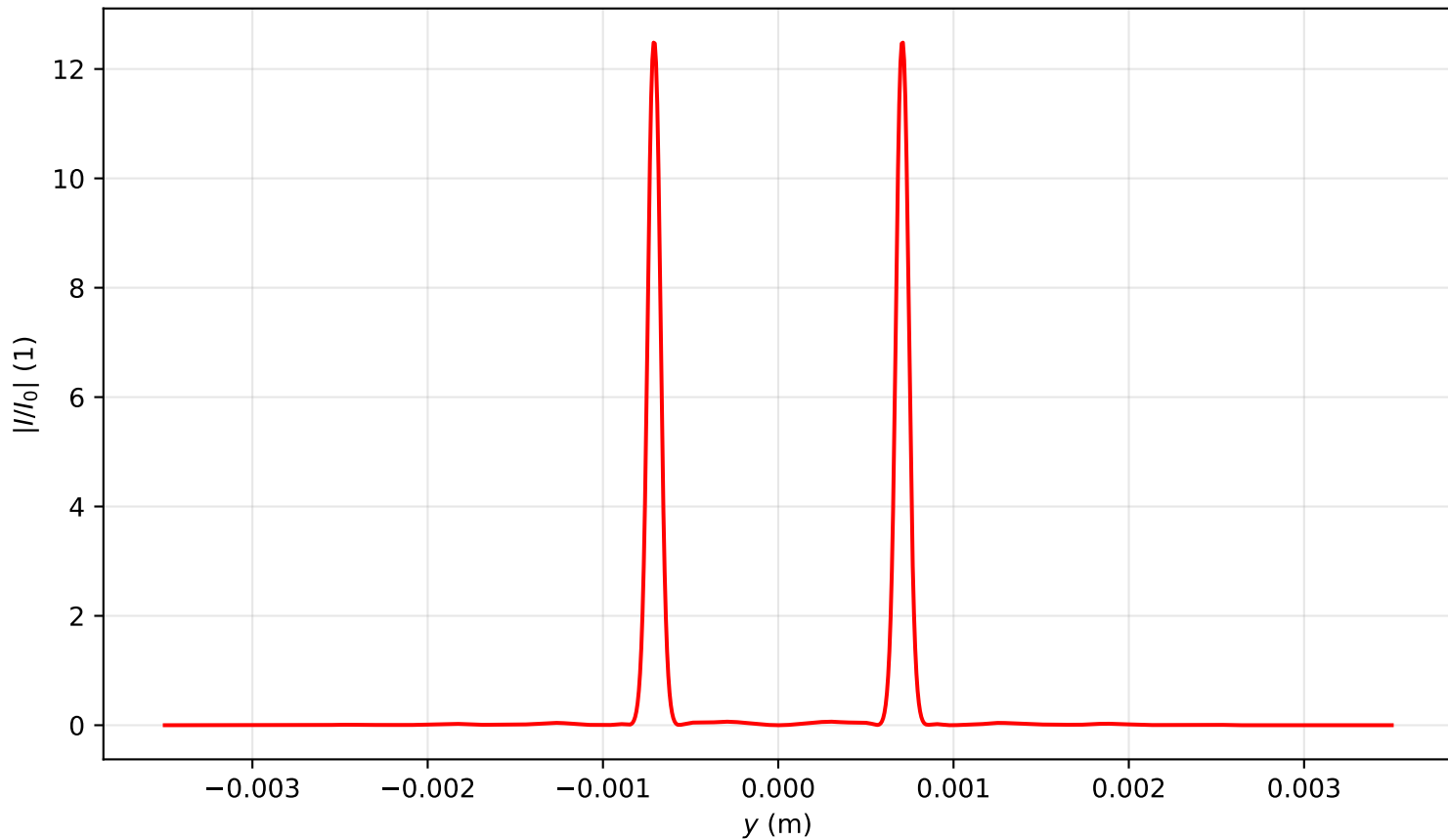
Intensity profile I(x = 0, y, z = 1.751)/I_0 , \text{Pin}=17.0\text{Pcr} , artificial time
