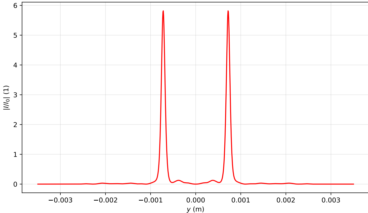
Intensity profile I(x=0, y, z=1.831)/I_0 , P_{in}=17.0\text{Pcr} , artificial time
