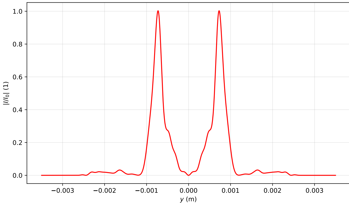
Intensity profile I(x=0, y, z=1.911)/I_0 , P_{in}=17.0P_{cr} , artificial time
