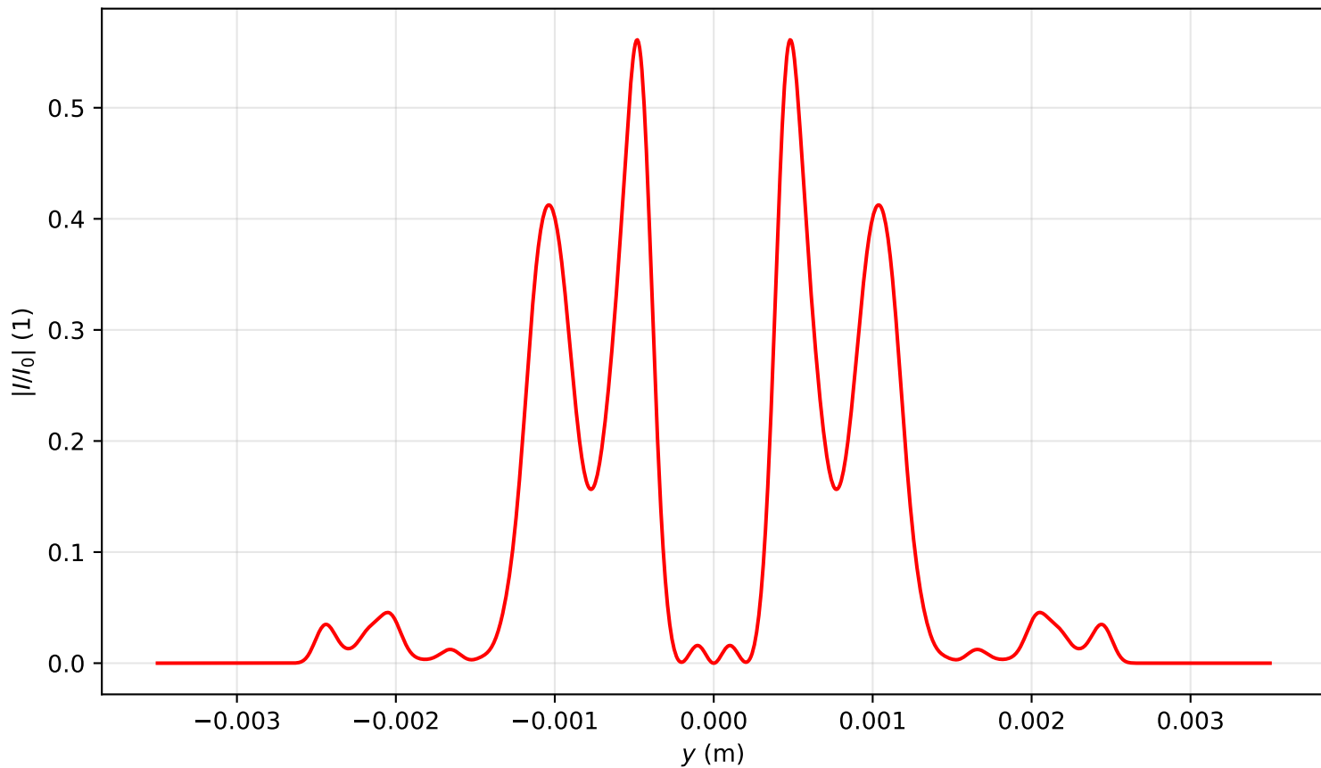
Intensity profile I(x=0, y, z=2.149)/I_0 , P_{in}=17.0P_{cr} , artificial time
