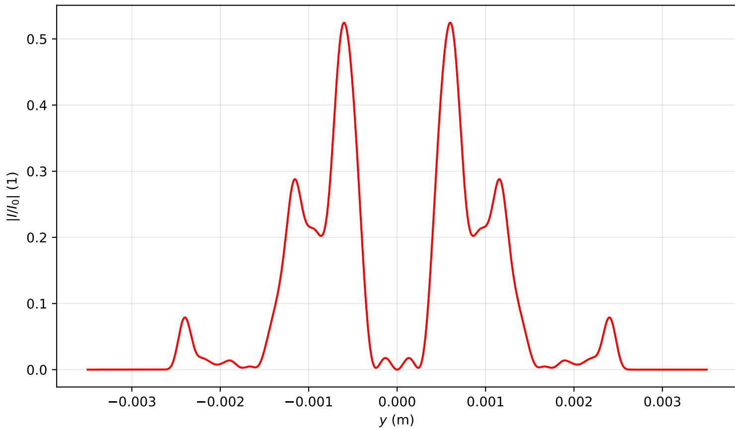
Intensity profile I(x=0, y, z=2.309)/I_0 , P_{in}=17.0\text{Pcr} , artificial time
