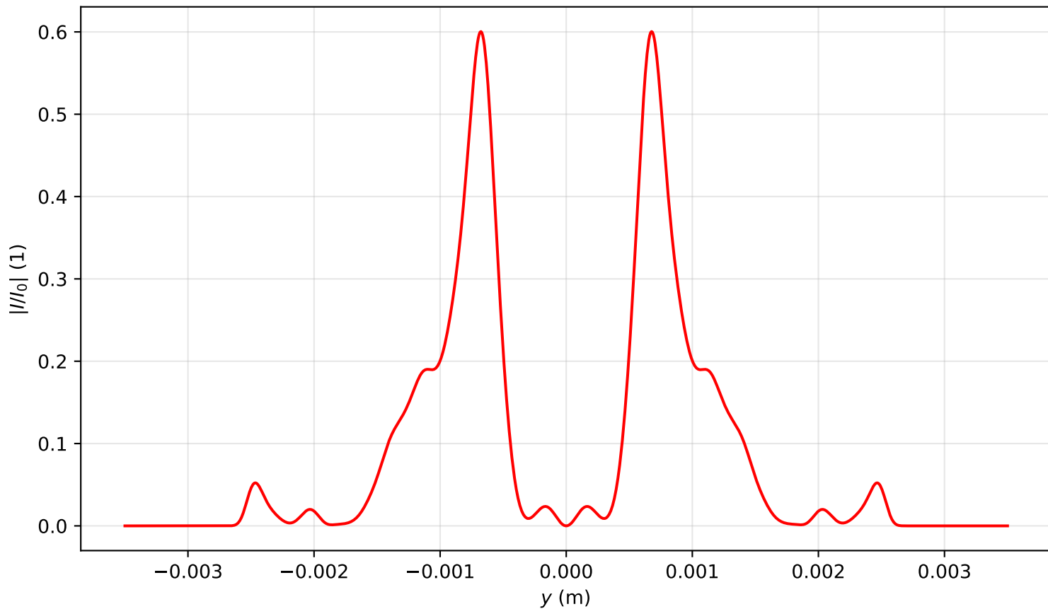
Intensity profile I(x=0, y, z=2.468)/I_0 , P_{in}=17.0P_{cr} , artificial time
