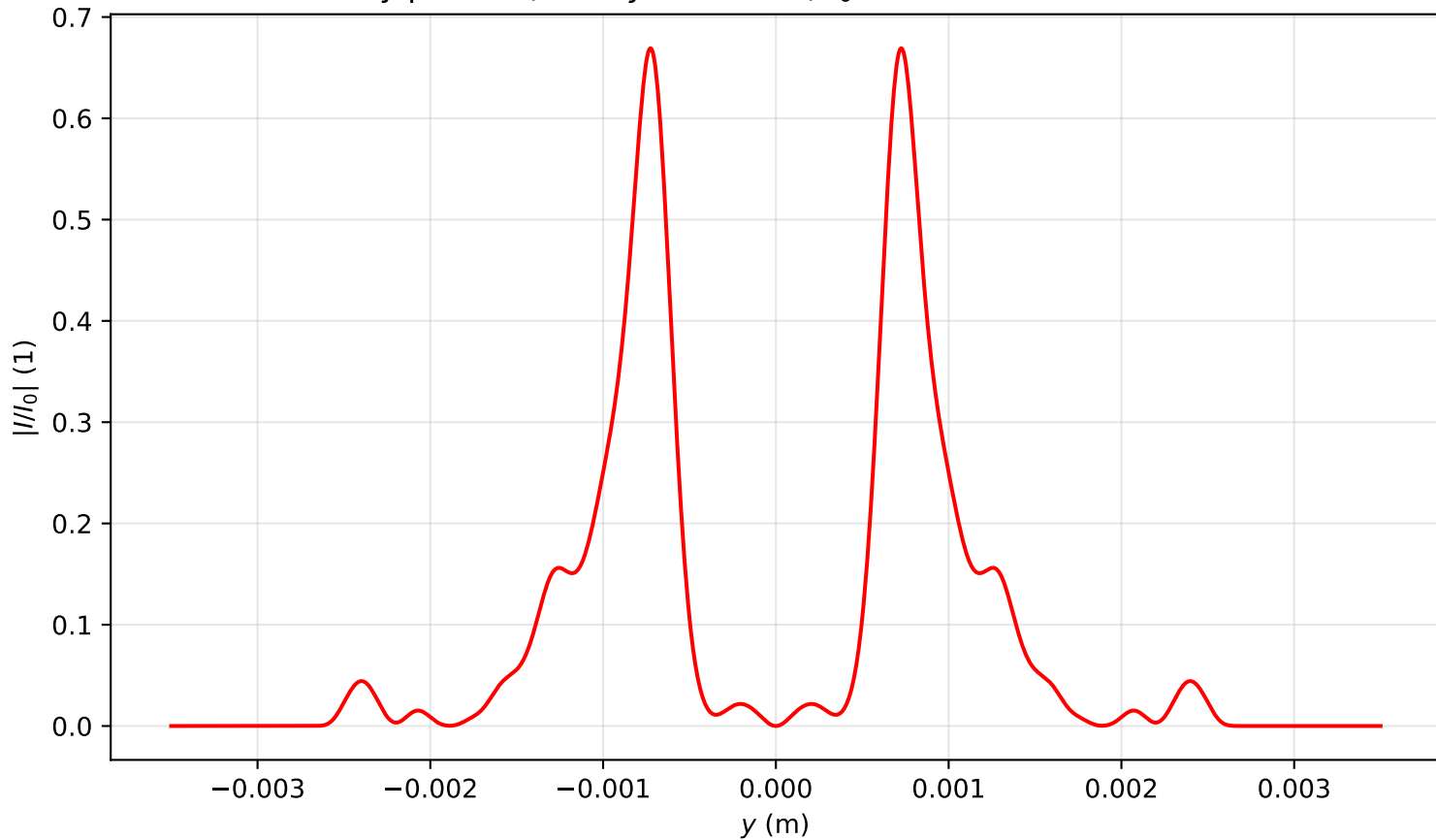
Intensity profile I(x=0, y, z=2.548)/I_0 , P_{in}=17.0\text{Pcr} , artificial time
