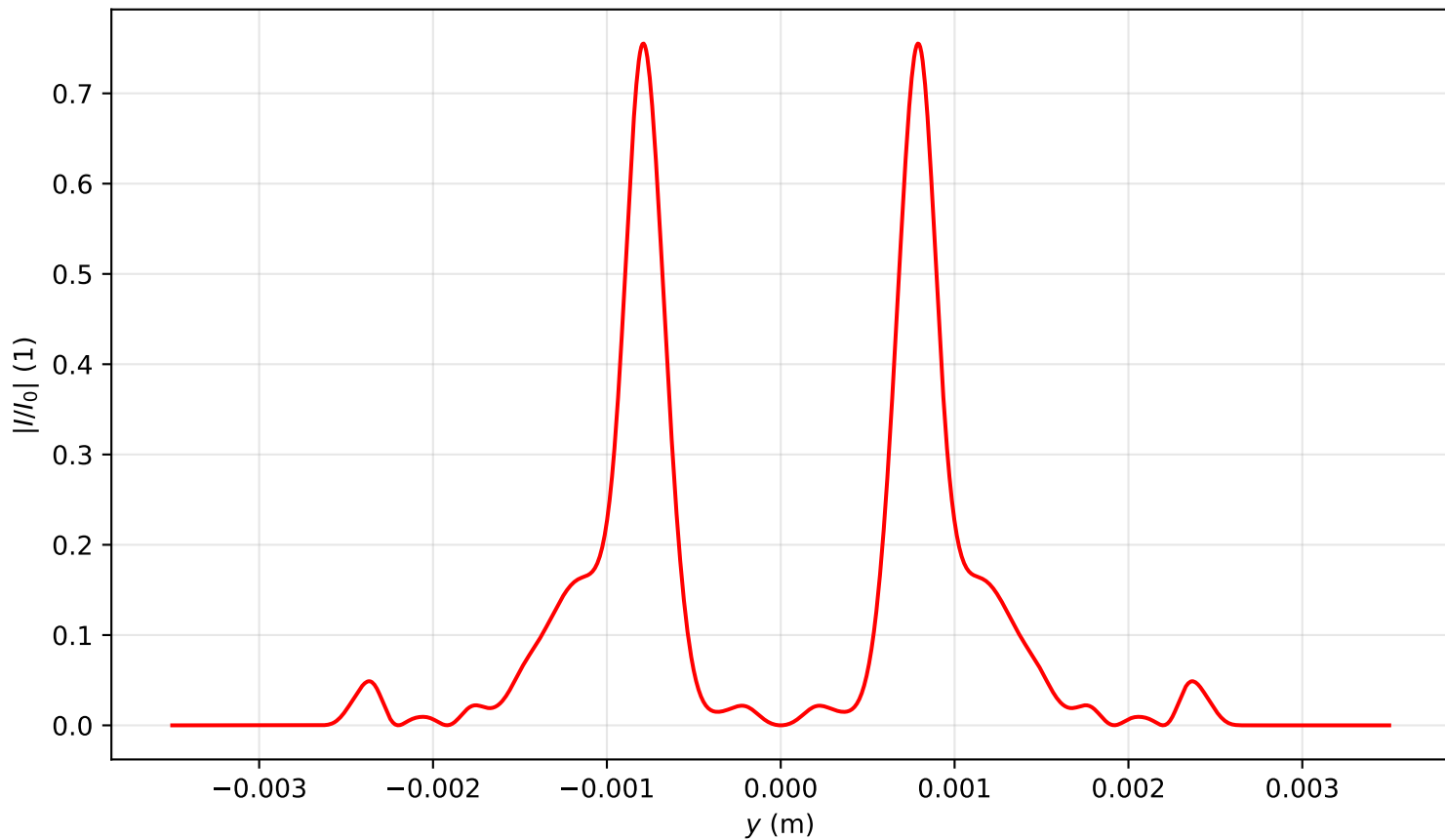
Intensity profile I(x=0, y, z=2.627)/I_0 , P_{in}=17.0\text{Pcr} , artificial time
