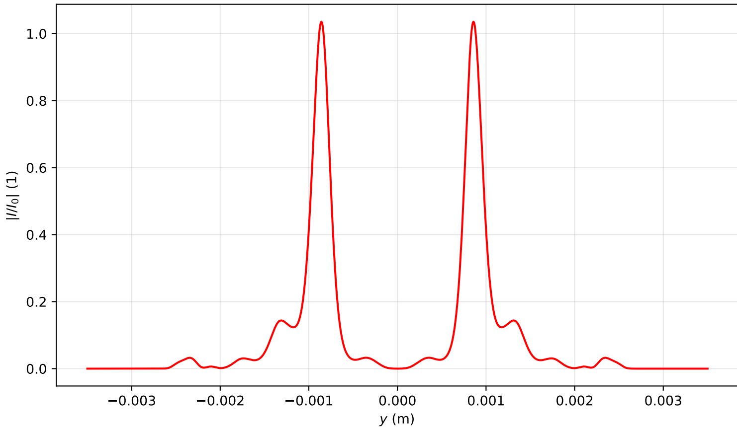
Intensity profile I(x=0, y, z=2.786)/I_0 , P_{in}=17.0\text{Pcr} , artificial time
